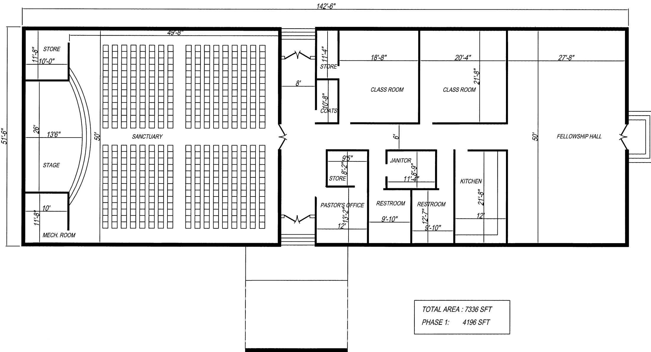
PROPOSED CHURCH PLAN FOR PASTOR PALMER.
